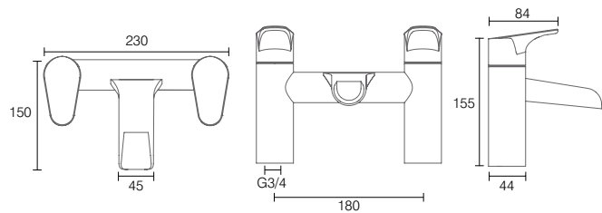
Open Spout Bath Filler chrome LA1003 £303
