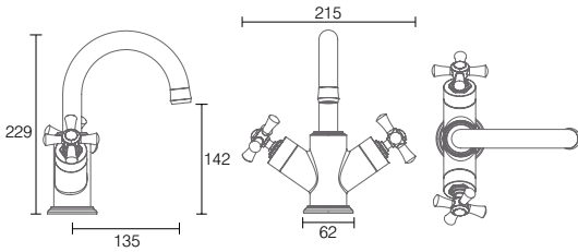
Basin Mixer with Click Waste chrome LA1009 £208
