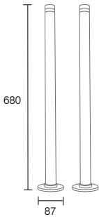
Stand Pipes W87mm x H680mm chrome LA17003 £322
