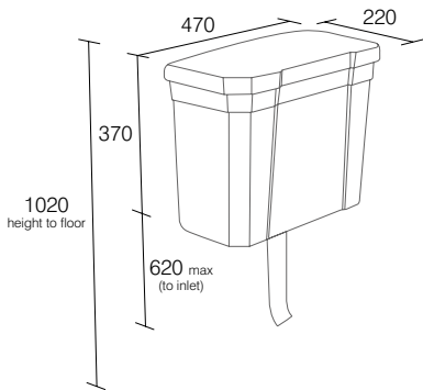
Low Level Cistern 6/4L & Chrome Pipe ceramic LA9117 £268
