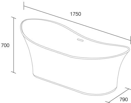
1750 Bateau Bath L1750mm x W790mm x H700mm LA16007 £1,750 includes integrated overflow and 1½" click waste no tap holes, suitable for freestanding or wall mounted taps only water capacity 215 litres to overflow weight (unfilled) 53 kilograms material double skinned 4mm acrylic with resin reinforcement
