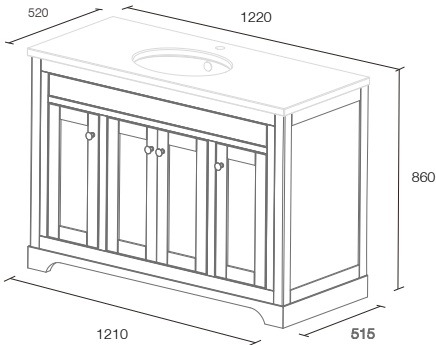
1200mm Freestanding Basin Unit cotton white LA13103 £1,220 cobblestone LA13104 £1,220 charcoal LA13105 £1,220 (excludes worktop & basin)
