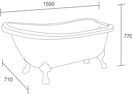
1550 Single Ended Slipper Bath L1550mm x W710mm x H770mm LA16003 £940 undrilled tap deck water capacity 160 litres to overflow weight (unfilled) 39 kilograms material double skinned 4mm acrylic with resin reinforcement
