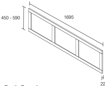
Bath Panel 1700mm Front Panel W1695mm x H450 - 590mm x D22mm cotton white LA5022 £158.50 cobblestone LA5024 £158.50 charcoal LA5026 £158.50 steel grey LA5028 £158.50
