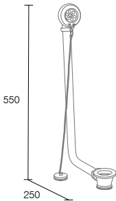
Exposed Chain Waste W250mm x H550mm 1½" waste chrome LA17001 £111.50
